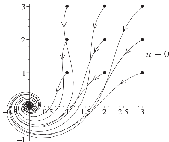
Figure 4.4: Integral curves of x'_1 = -x_1 + 2tx_2 , x'_2 = -2tx_1 - x_2 which start at c = (i, j) , i, j = 1, 2, 3 , at time u = 0 .
