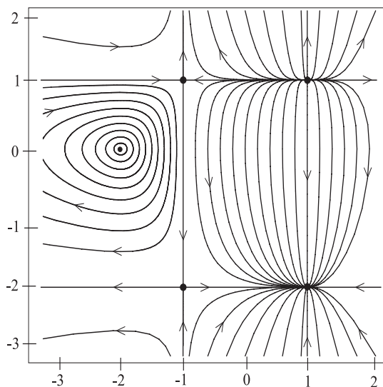
Figure 2.10: The phase portrait for the system (2.3)-(2.4).
