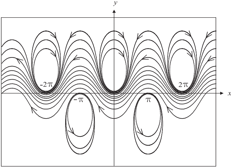
Figure 1.3: Solution curves of the system (1.5)-(1.6) which represents a fluid flow past two rows of vortices with opposite circulations.
