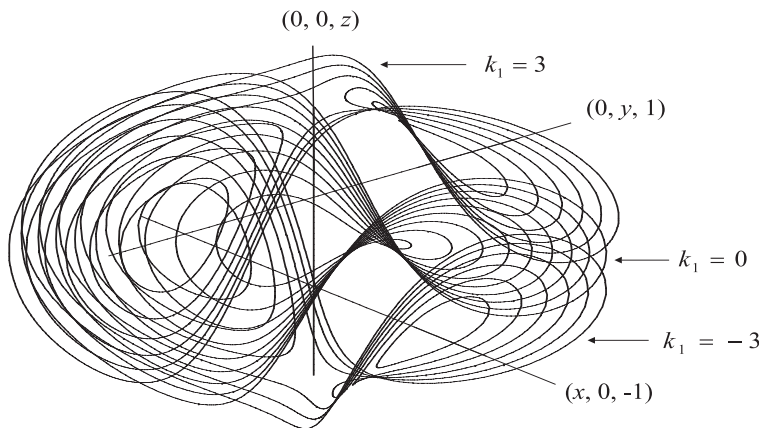
Figure 7.15: Three lines of fixed points for the system x' = y(z - 1) , y' = x(z + 1) , z' = 2xy . The other integral curves shown lie on the hyperbolic paraboloids z = \frac{1}{2}(x^2 - y^2) + k_1 , for k_1 = -3, 0, 3 .
