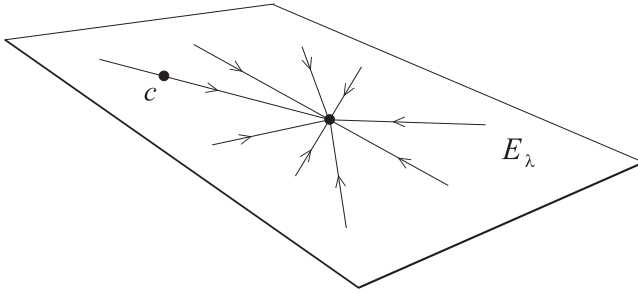
Figure 4.7: The integral curve passing through a point c \in E_\lambda , is a half-ray, contained completely in E_\lambda . The ray is directed toward the origin if \lambda < 0 and away from the origin if \lambda > 0 . E_\lambda is comprised entirely of such rays. The picture is for the case when E_\lambda is two-dimensional.
