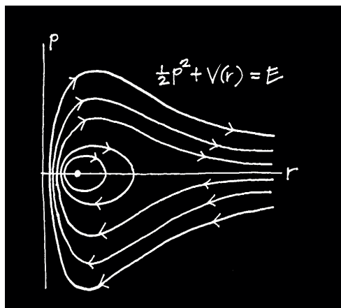
Figure 8.15: A sketch of the energy curves p^2/2m + V(r) = E , for various values of E . Here V has graph as shown in Figure 8.13 and m = 1 .
