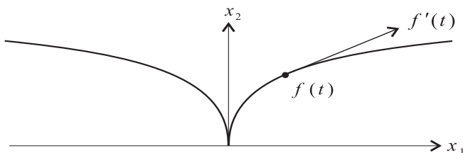
Figure A.1: The curve f(t) = (t^3, t^2) .
