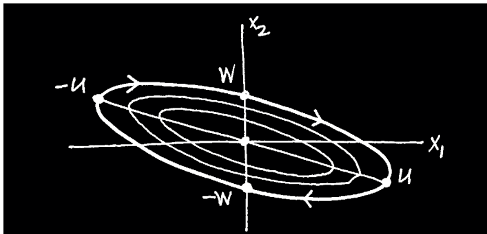
Figure 4.15: Hand-drawn sketch of the phase portrait for the system x'_1 = x_1 + 5x_2 , x'_2 = -x_1 - x_2 .
