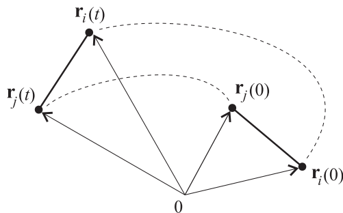
Figure 8.24: The distances between the bodies in the system remain constant in a rigid-body motion.
