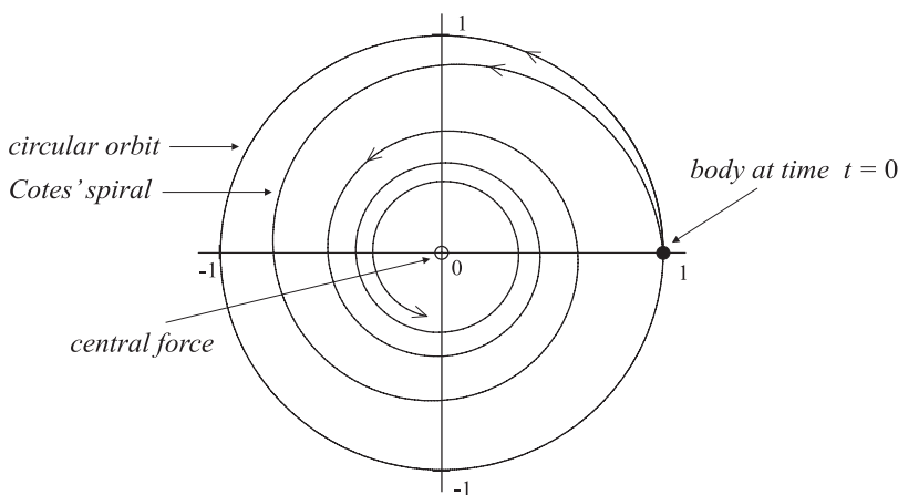
Figure 2.19: Plots of two trajectories (x(t), y(t)) for a body attracted toward the origin with a inverse cube law of force. While the initial positions are the same, the initial velocities are (x'_0, y'_0) = (0, 1), (-0.1, 1) .
