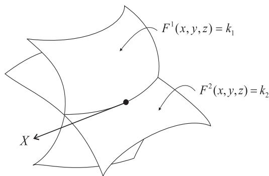
Figure 7.5: If a system has two independent first integrals F^1, F^2 , then each integral curve lies on the curve of intersection of two particular level surfaces F^1 = k_1, F^2 = k_2 .
