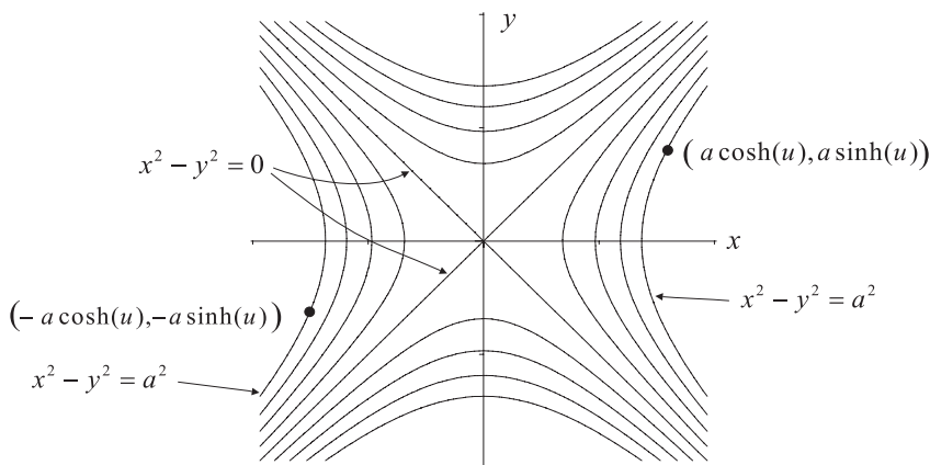
Figure 5.17: Hyperbolic coordinates on the plane.
